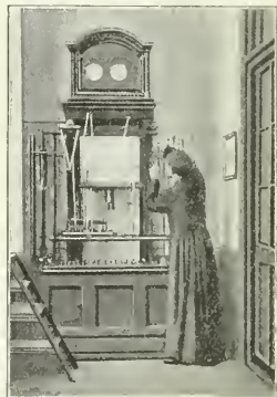
THE SECCI METEOROGRAPH IN THE OBSERVATORY AT ZI-KA-WEI
